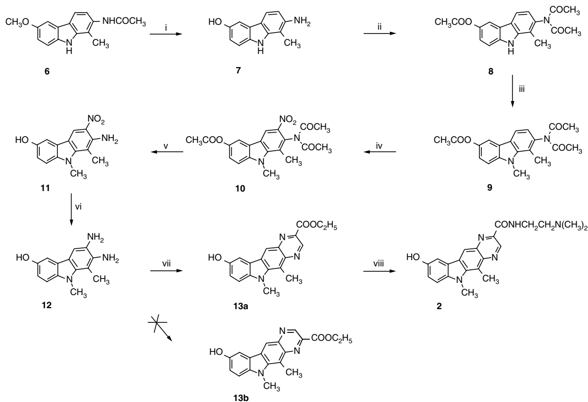
Scheme 1. Synthesis of pyrazocarbazole 2 : (i) 48% HBr (94%); (ii) \text{Ac}_2\text{O} (62%); (iii) NaH, \text{CH}_3\text{I} , DMF (64%); (iv) \text{HNO}_3 (53%); (v) NaOH, \text{C}_2\text{H}_5\text{OH} (100%); (vi) \text{H}_2 -Ni, NMP (100%); (vii) \text{BrCH}_2\text{COCOOC}_2\text{H}_5 , \text{N}(\text{C}_2\text{H}_5)_3 , NMP (29%); (viii) \text{H}_2\text{N}(\text{CH}_2)_2\text{N}(\text{CH}_3)_2 (44%).
